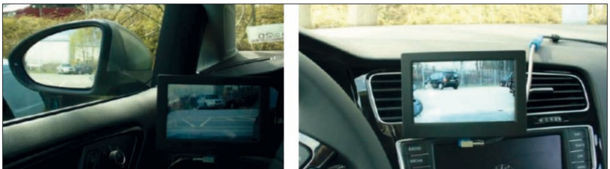
Fig. 5: Integration of the monitors on the air vent grids (Position CMS 2)
