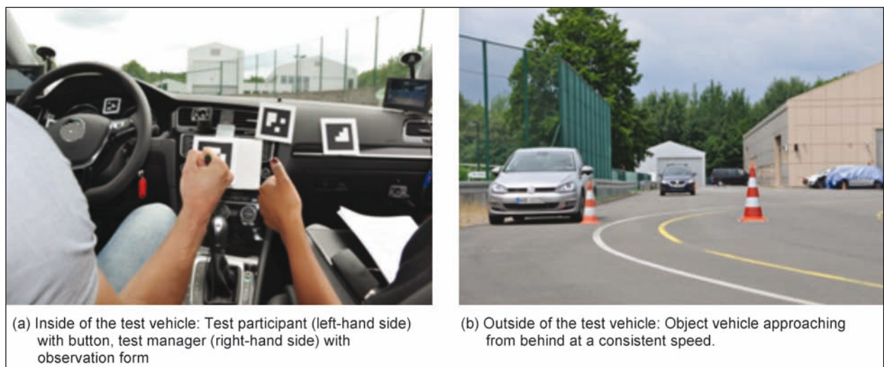
Fig. 59: Static test vehicle at the test facilities of BAST
