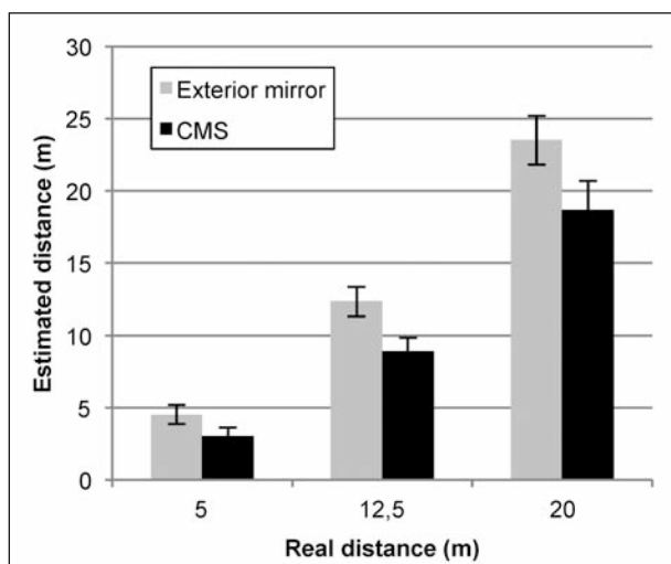
Fig. 62: Estimated distances to a stationary object vehicle using the exterior mirror and the CMS
