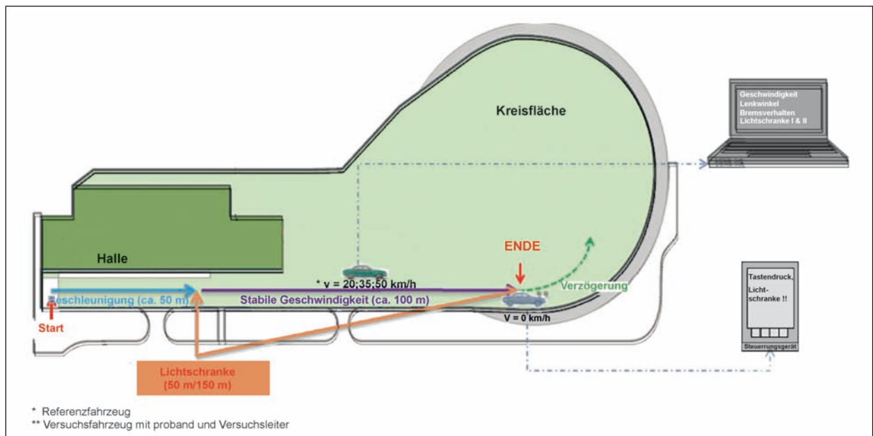
Fig. 58: Schematic test set-up for distance and speed estimation of an approaching object vehicle at the test facilities of BAST
