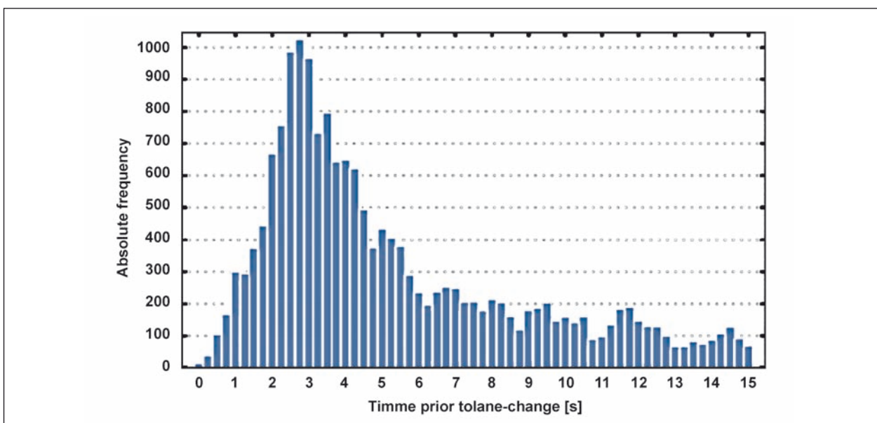
Fig. 2: Temporal distribution and absolute frequency of glances into the left exterior mirror within the last 15 seconds prior to the actual lane-changing. According to LIEBNER et al. (2010)
