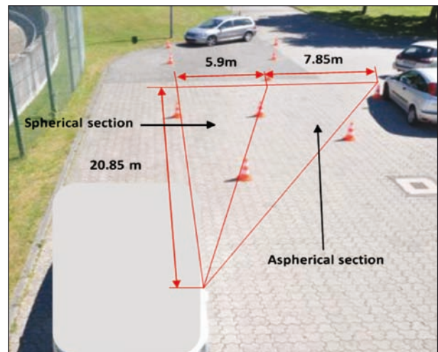
Fig. 12: CMS field of vision
