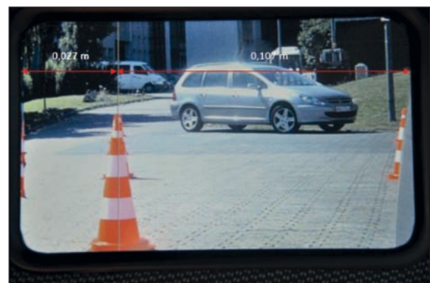
Fig. 13: Monitor view with lateral monitor dimensions
