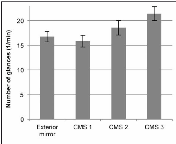
Fig. 63: Number of glances per minute when merging into moving traffic, for different monitor/mirror positions
