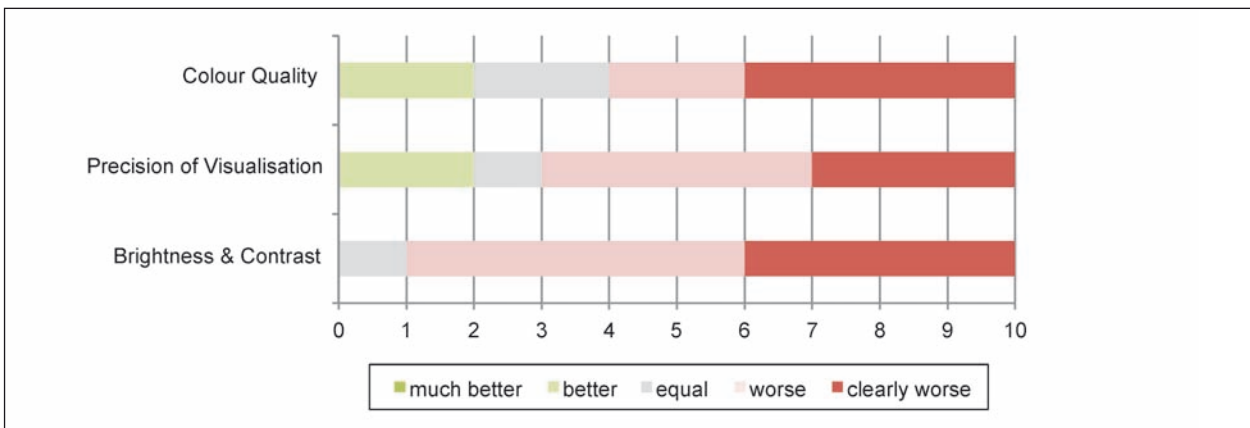
Fig. 78: Comparison between CMS with exterior mirrors with regard to image quality
