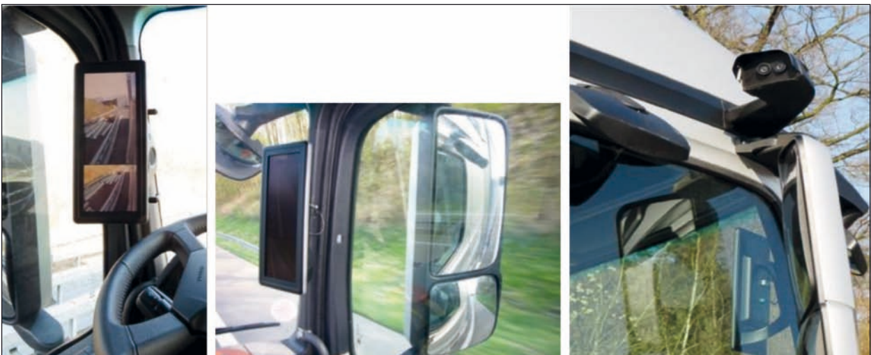
Fig. 9: Exterior mirrors with cameras and monitor integration next to the A-pillar on a truck
