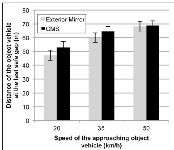
Fig. 61: Last safe gap estimated by the subjects for the two system types. The distance between the moving object vehicle and the static test vehicle was measured at the time the button was pressed ( N = 34 )
