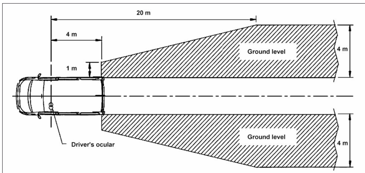
Fig. 1: Prescribed field of vision for Class III (UN-R 46) mirrors, i.e. for small exterior mirrors
