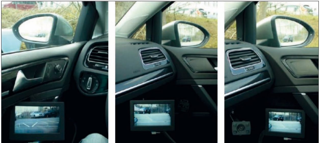
Fig. 4: Integration of the monitors in the driver and passenger door (Position CMS 1)
