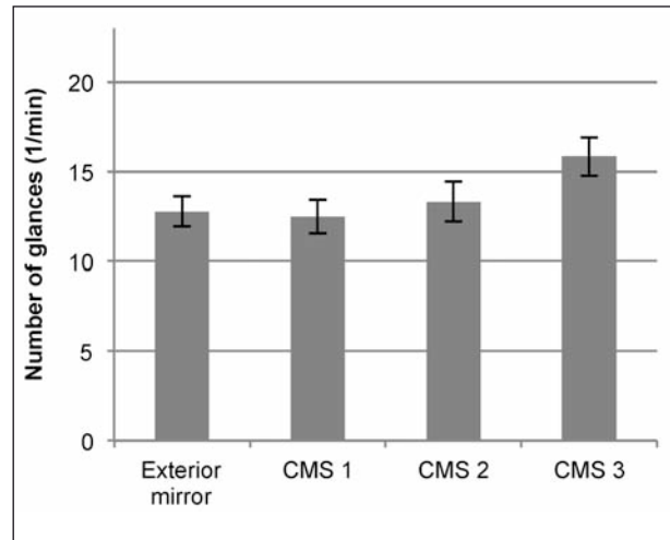
Fig. 65: Number of glances per minute during overtaking, for different monitor/mirror positions
